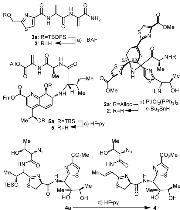
Figure 2. Synthesis of thiostrepton fragments 2–5. Reagents and conditions: (a) TBAF (1.2 equiv), THF, 0 °C, 30 min, 90%; (b) PdCl 2 (PPh 3 ) 2 (0.1 equiv), n -Bu 3 SnH (50 equiv), CH 2 Cl 2 , –45 °C, 10 min, then 0 °C, 30 min, 100%; (c) HF·py:THF (1:4), 0 °C, 5 min, then 25 °C, 24 h, 70%; (d) HF·py (1:4), THF, 0 °C, 5 min, then 25 °C, 18 h, 78%. TBDPS = tert -butyl diphenylsilyl; TBAF = tetra- n -butylammonium fluoride; Alloc = allyloxy carbonyl; Ph = phenyl; TBS = tert -butyl dimethylsilyl; Fm = fluorenylmethyl; All = allyl; py = pyridine.
