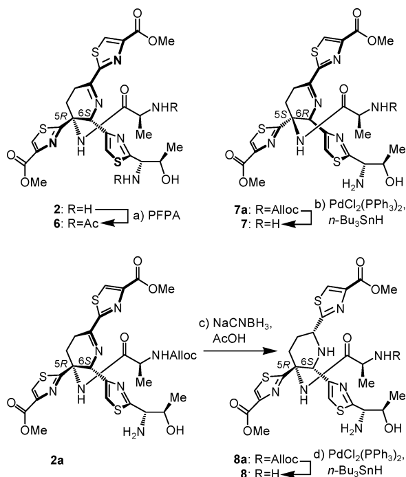
Figure 3. Synthesis of thiostrepton fragments 6–8. Reagents and conditions: (a) pentafluorophenol acetate (5.0 equiv), DMF, 25 °C, 18 h, 73%; (b) PdCl 2 (PPh 3 ) 2 (0.1 equiv), n -Bu 3 SnH (50 equiv), CH 2 Cl 2 , –45 °C, 10 min, then 0 °C, 30 min, 100%; (c) NaCNBH 3 (4.0 equiv), EtOH:AcOH (4:1), 0 °C, 1 h, 67%; (d) PdCl 2 (PPh 3 ) 2 (0.1 equiv), n -Bu 3 SnH (3.4 equiv), CH 2 Cl 2 , 0 °C, 30 min, 85%. PFPFA = pentafluorophenol acetate; AcOH = acetic acid.
